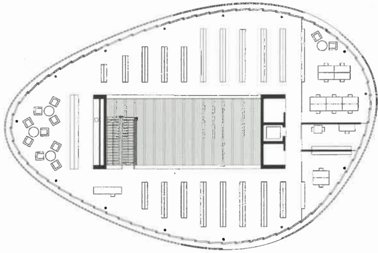
Grundriss Erdgeschoss • Ground floor plan
